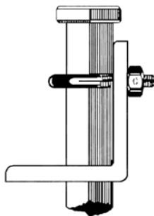
CLAMP ATTACHMENT
